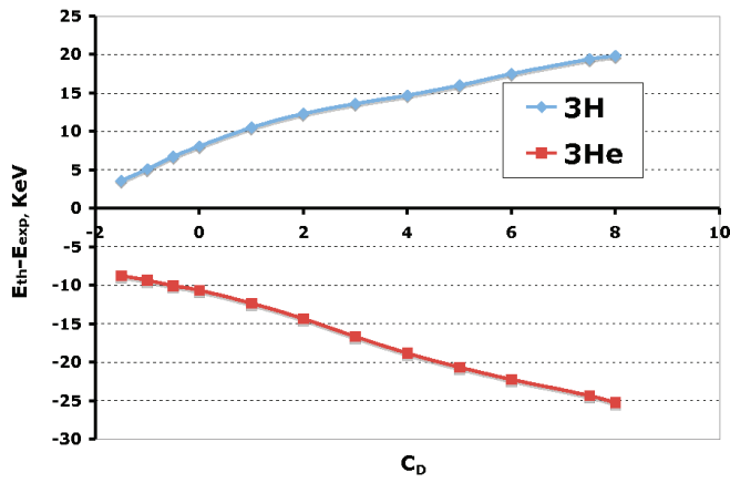
Figure 2. Deviation of the binding energy of the three-nucleon systems as computed along the averaged c_D - c_E curve.
