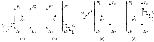
Figure 2. Two-body correlation currents.
