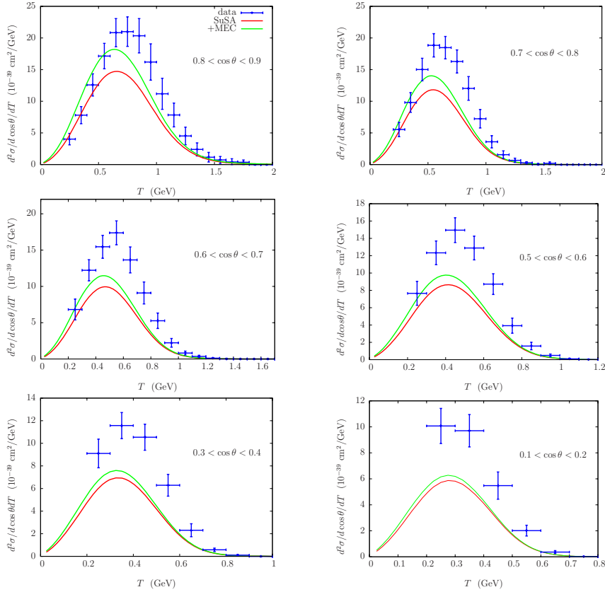
Figure 4. Flux-integrated \nu_\mu - ^{12}\text{C} CCQE double differential cross section per target nucleon evaluated in the SuSA model with and without inclusion of 2p2h MEC displayed versus the muon kinetic energy T_\mu for various bins of the muon scattering angle \cos \theta . Here and in the following figures the data are from MiniBooNE [1].
