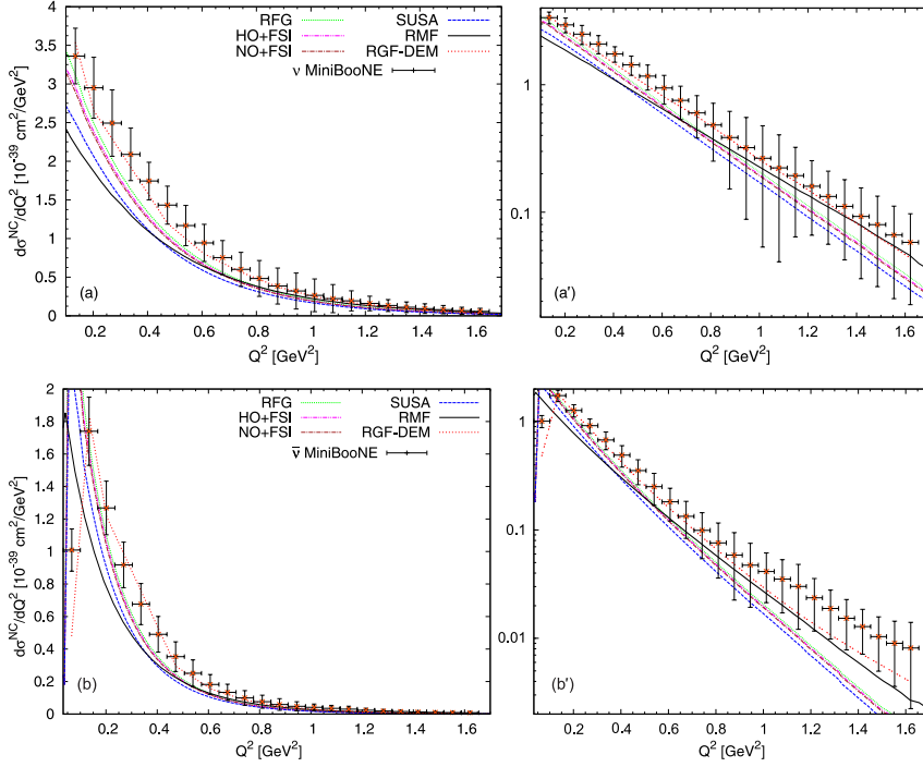
Figure 2. (Color online) NCQE neutrino [panels (a) and (a'), \nu N \rightarrow \nu N ] and antineutrino [panels (b) and (b'), \bar{\nu} N \rightarrow \bar{\nu} N ] flux-averaged differential cross section computed using the RFG, HO+FSI, NO+FSI, SUSA scaling functions, RGF and RMF models and compared with the MiniBooNE data [2, 5]. The results correspond to the world-average axial mass M_A = 1.032 GeV and strangeness \Delta s = 0 . The error bars do not account for the normalization uncertainty of 18.1% (19.5%) in the \nu(\bar{\nu}) case.
